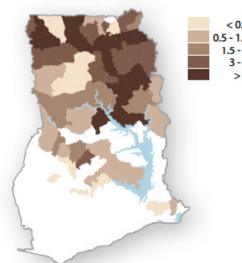
Cowpea
