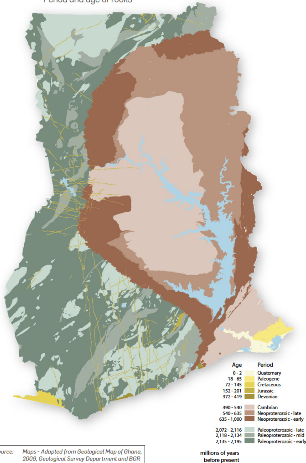
Period and age of rocks
