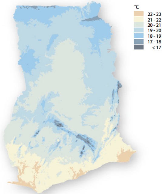
Minimum temperature
