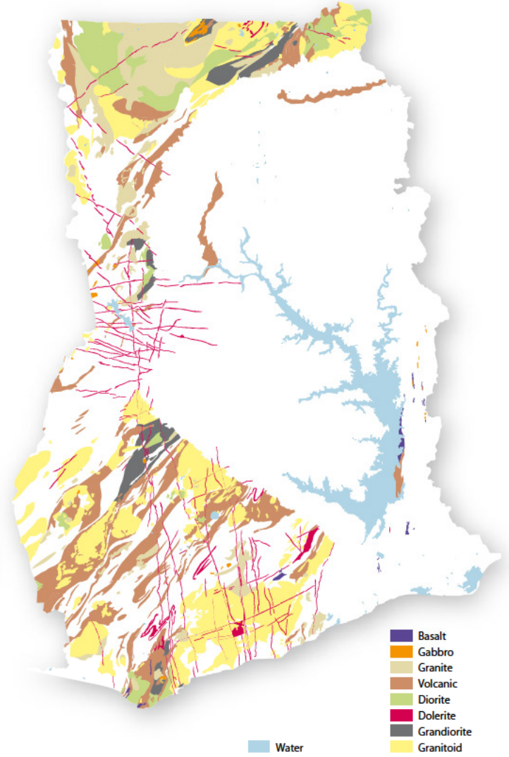
Igneous
