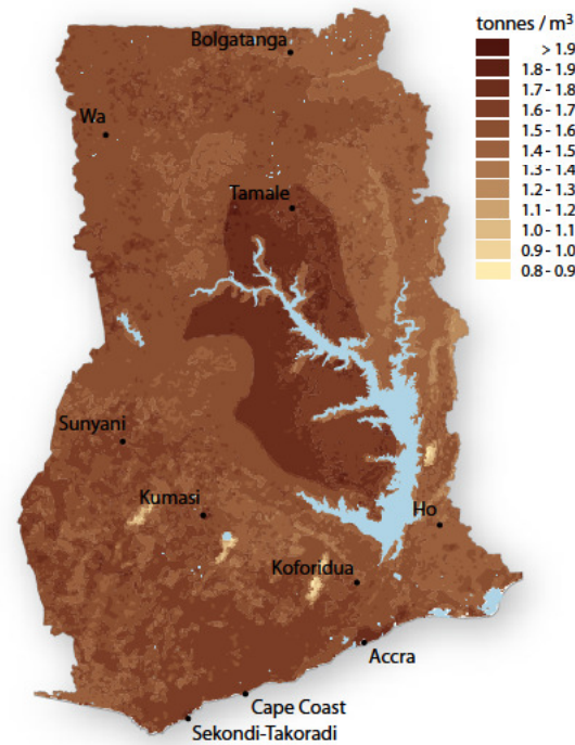
Bulk density
