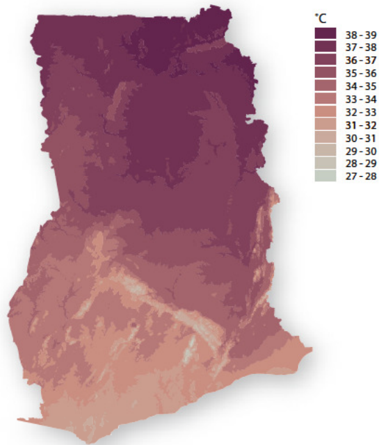
Maximum temperature
