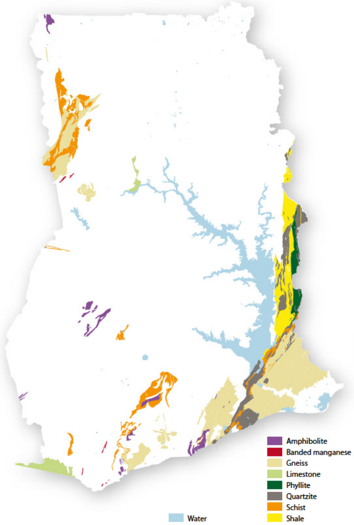
Metamorphic
