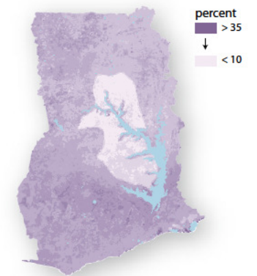
Clay content
