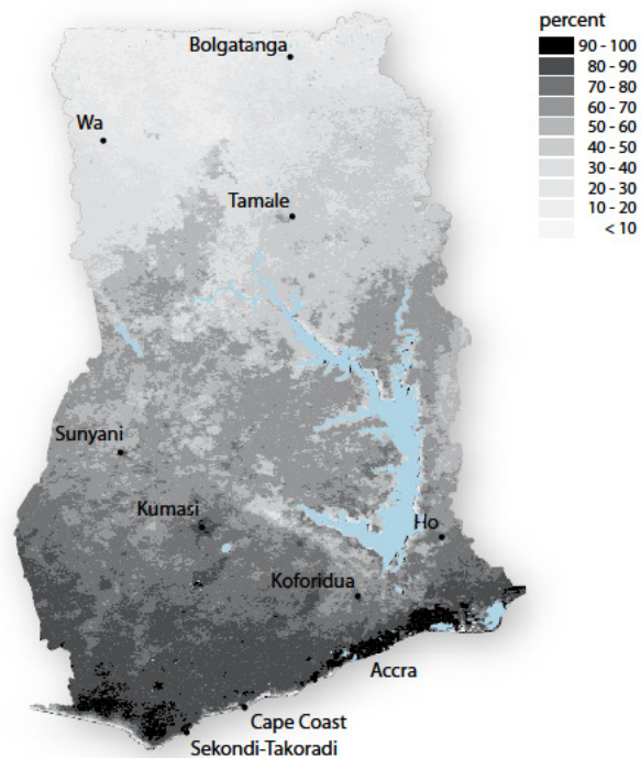
Cloudy months
