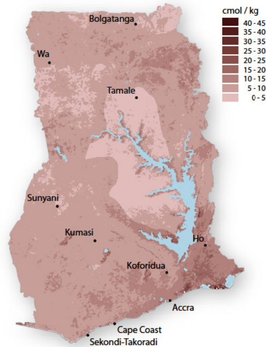
Cation exchange capacity
