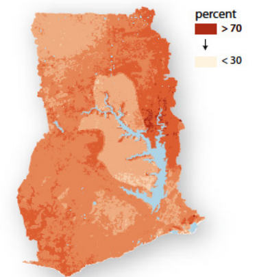
Sand content
