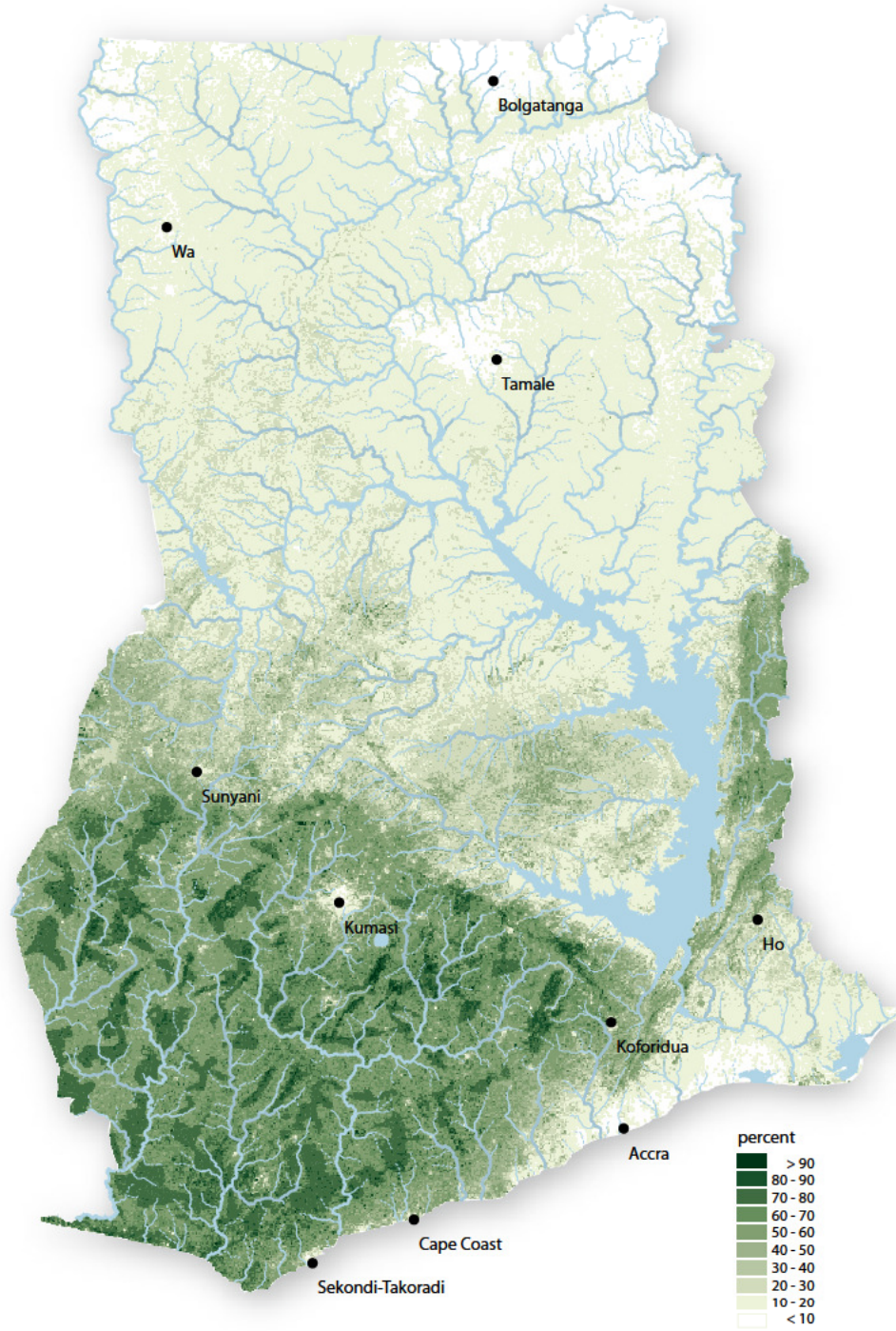
Forest cover in 2000
