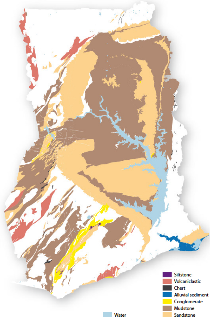
Sedimentary
