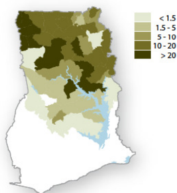
Groundnut
