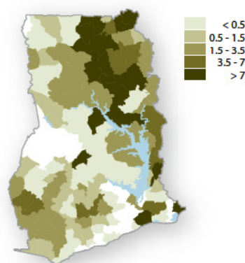
Rice
